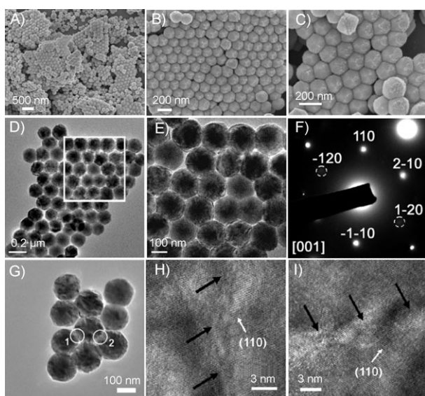
Figure 2. A–C) SEM and D–F) TEM images of sample II. E) A magnified image of the region marked by a white square in (D). F) The selected-area electron diffraction (SAED) pattern of sample II. H, I) HRTEM images of the regions 1 and 2 (marked by white circles) in (G). The black arrows indicate the particle boundaries.
